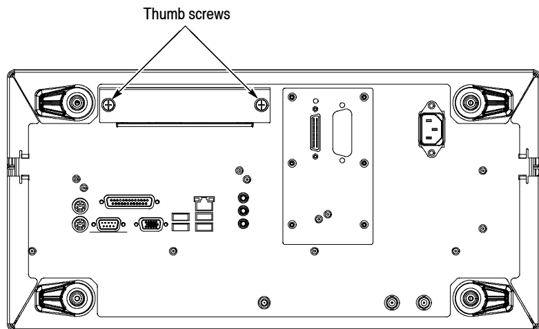
AWG7000 series rear panel
